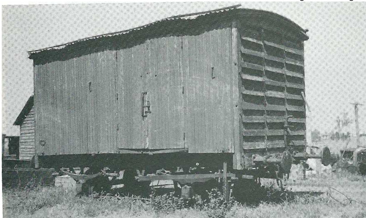
This Q.R. wagon was an A class, thought to be a rebuild of the 3442/3443 series (Q.R. drg 1088) It has Offset double doors, so may have been an ARO Wagon with Louvered end walls. The completed model uses Hook and Chain couplings as do all BTR 4 wheel Wagons.
