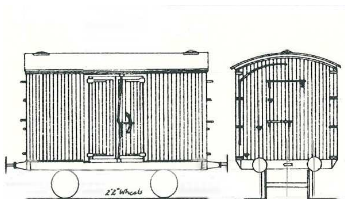
A typical Q.R. drawing used to make the model.
